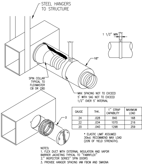
0 01 SCALE SUPPORT REQUIREMENTS FOR DUCT NTS
