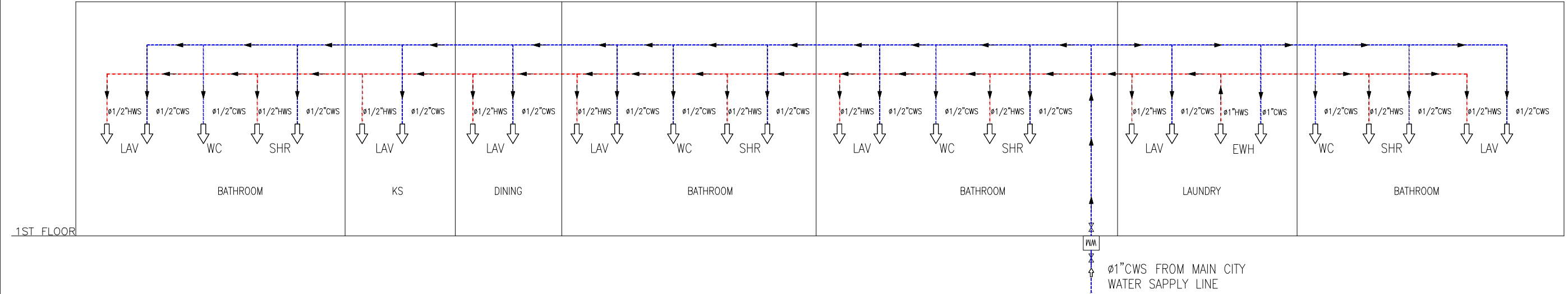
PL 04 WATER SUPPLY SYSTEM RISER DIAGRAM SCALE NTS
