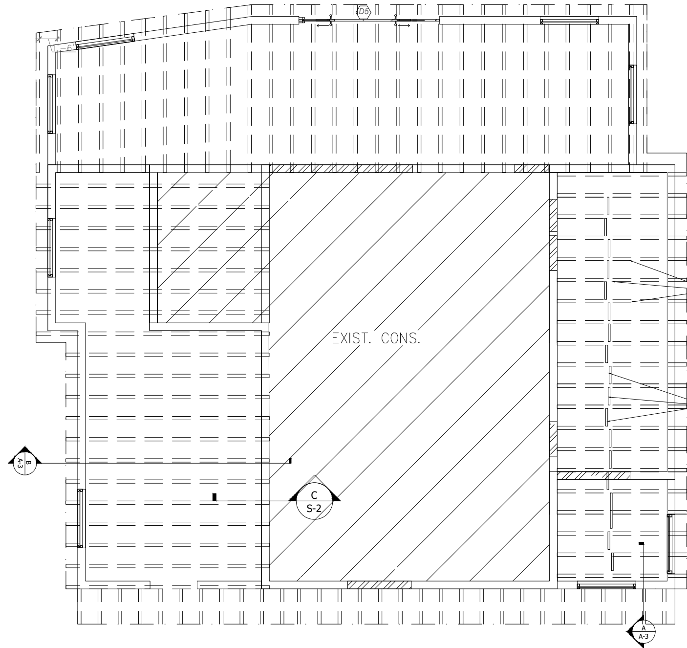
ROOF FRAMING PLAN SCALE: 1/8"=1'-0"
