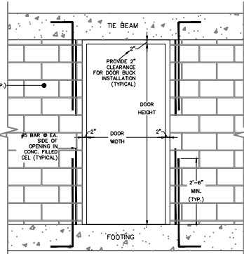
DOOR ROUGH OPENING IN NEW WALL DETAIL
