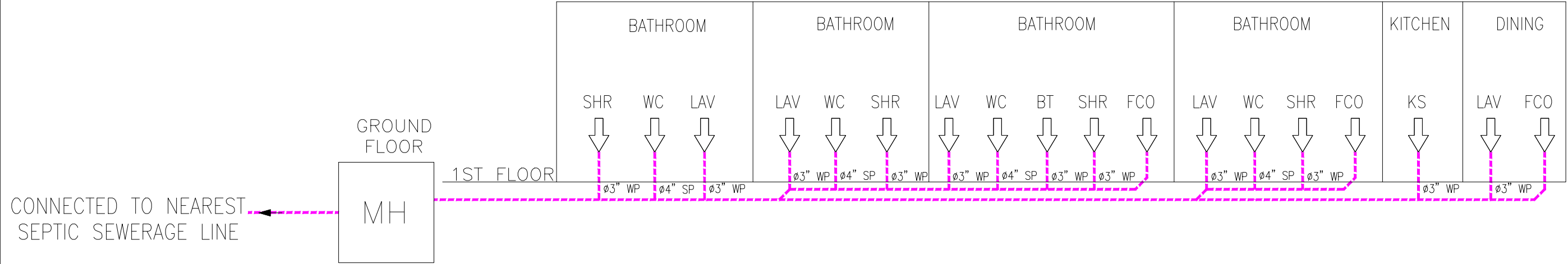
PL 04 DRAINAGE SYSTEM RISER DIAGRAM SCALE NTS
