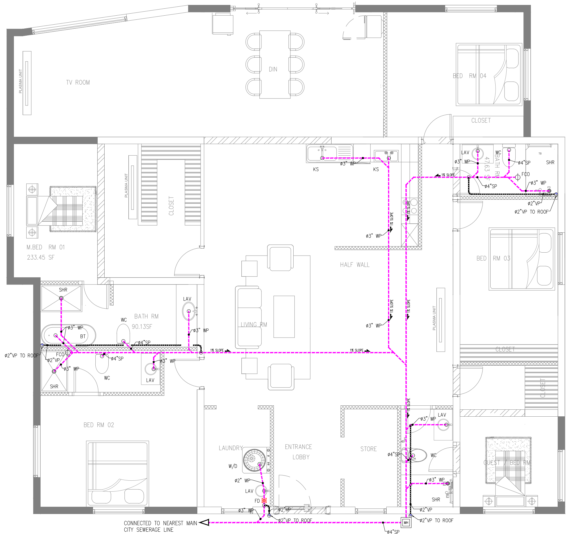
PL 02 DRAINAGE LAYOUT PLAN SCALE 3/16" = 1'-0"
