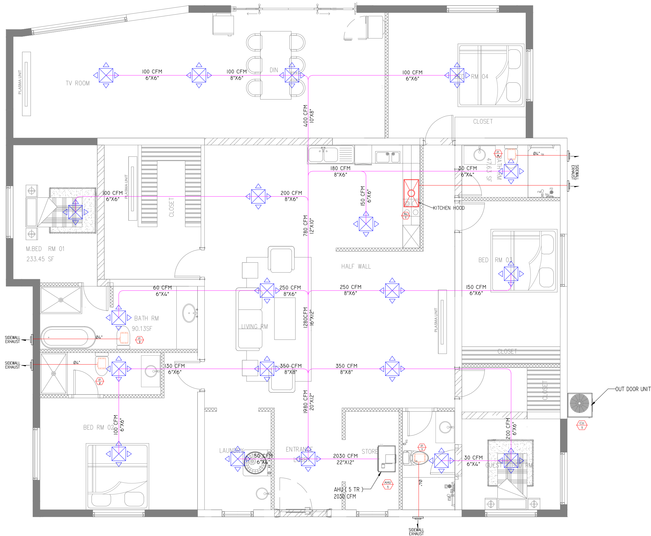
ME 02 HVAC LAYOUT PLAN SCALE 3/16" = 1'-0"
