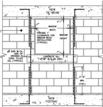
WINDOW ROUGH OPENING IN NEW WALL DETAIL
