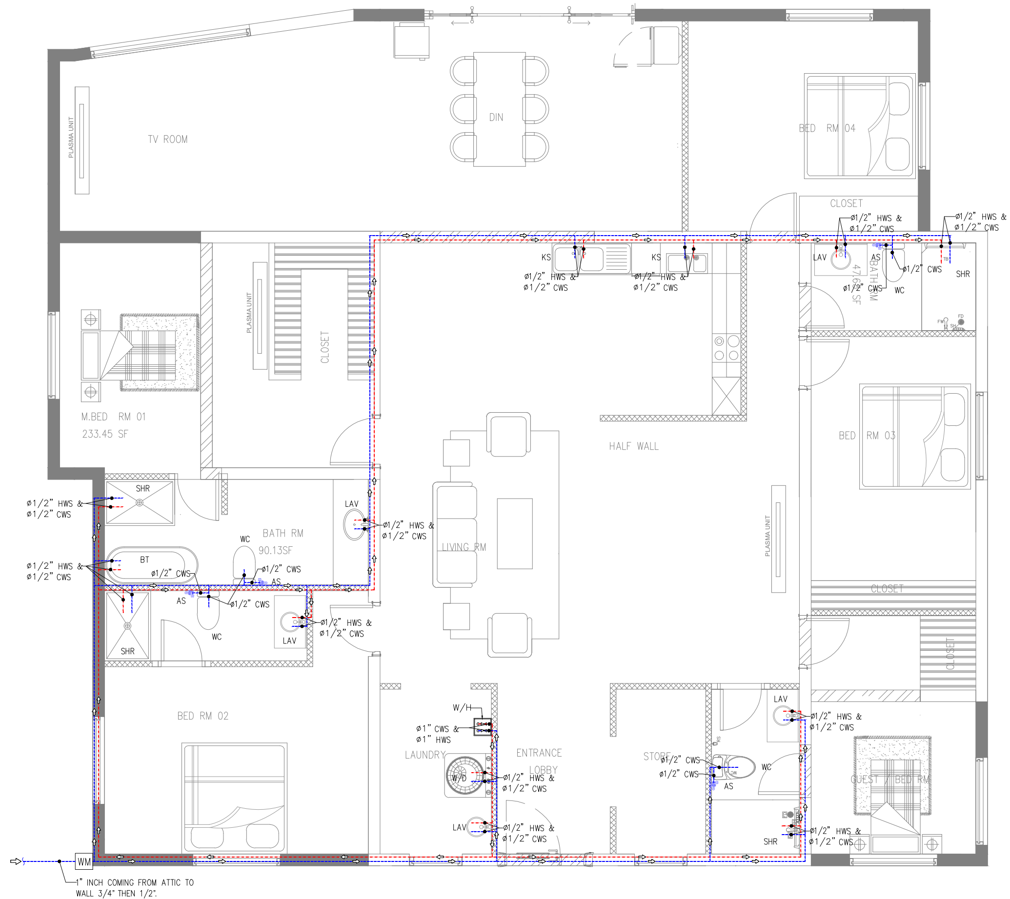
PL 03 WATER SUPPLY LAYOUT PLAN SCALE 3/16"=1'-0"
