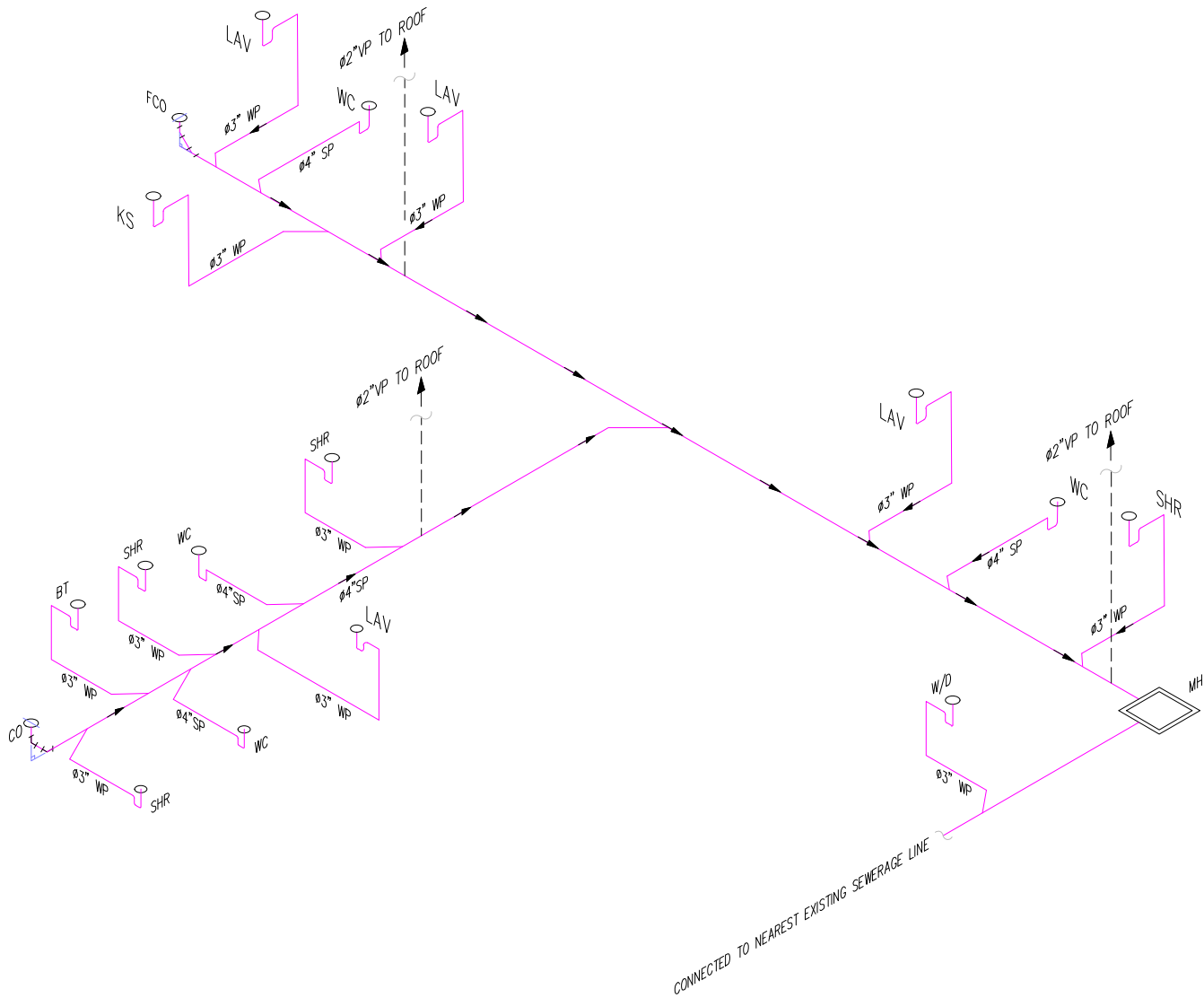
PL 04 SEWER ISOMETRIC VIEW SCALE NTS
